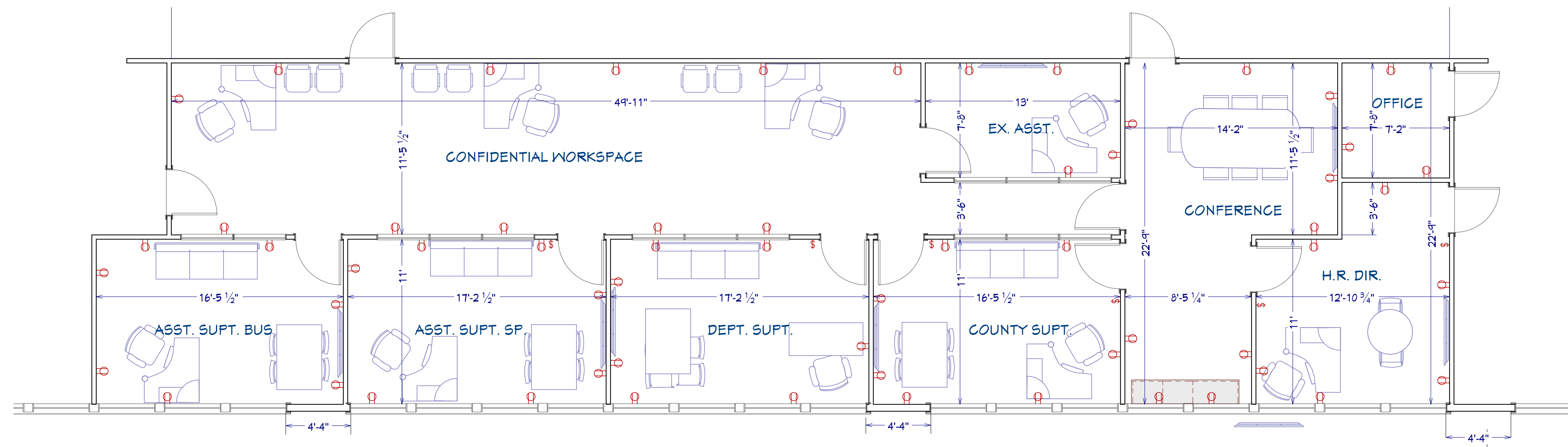
(F) FLOOR PLAN 1/4" = 1'-0"
